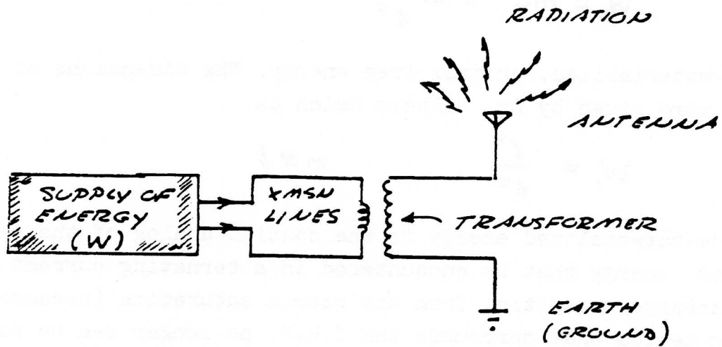
CONVENTIONAL RADIO SYSTEM
