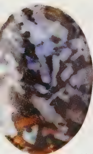
Gabbro with pyrite
