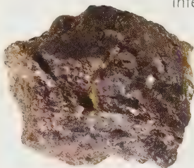
Pyrite with Sphalerite
