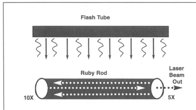
Figure 32-14: Red Photons travel down tube in phase as Coherent Light
